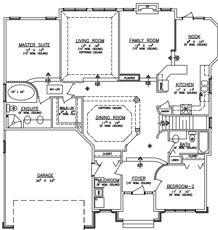
FLOOR PLAN
